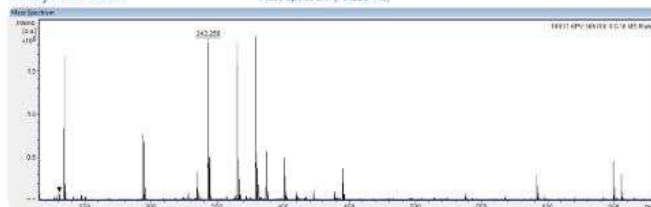
Mass Spectrum (MALDI-MS)
